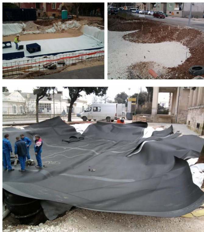
Figure 4. Construction of rain garden retentions of Nazorova Street [6]
