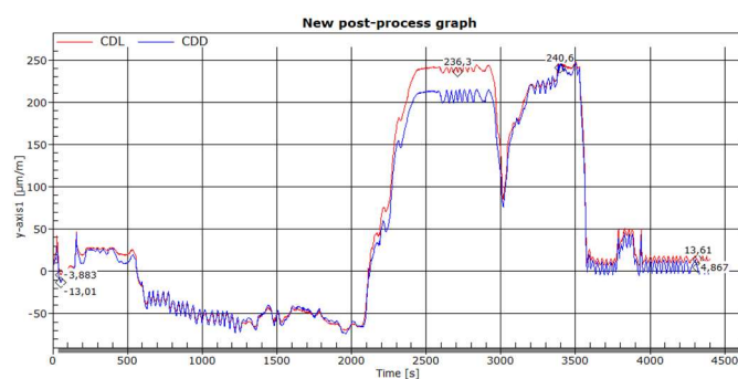
Figure 18. - Time history of strains for span 4 (steel - lower side)
