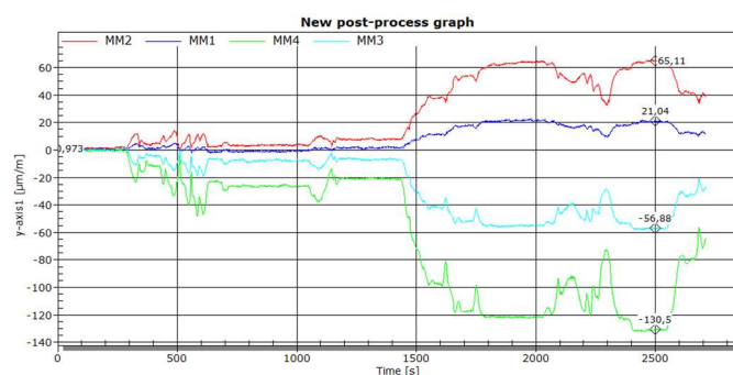
Figure 28. - Time history of strains for the change in flange and slab thickness – right
