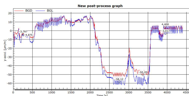
Figure 16. - Time history of strains for span 4 (concrete - upper side)
